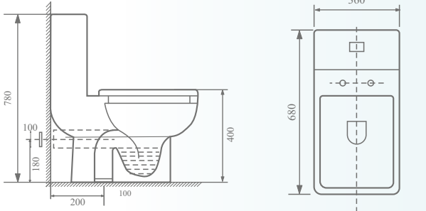
'S' Trap - 250 mm
