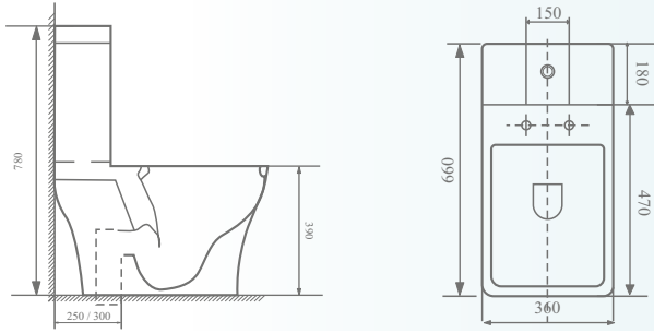
'S' Trap - 300 mm
