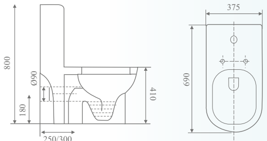
'S' Trap - 300 mm & 'P' Trap - 180 mm
