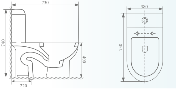
'S' Trap - 220 mm
