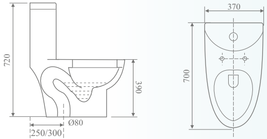
'S' Trap - 300/250 mm & 'P' Trap - 180 mm
