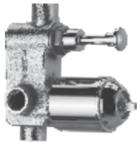
CDH 101 Concealed body for high flow single lever concealed diverter system consisting of 45 mm cartridge with button Assembly, Cartridge Sleeve and tip ton knob (but without operating lever and wall flange) (Suitable for CS 235E, CS 335E, CQ 335E, CS 135E, CQ 435E, CS 735E, CS 835E, CS 935E)
